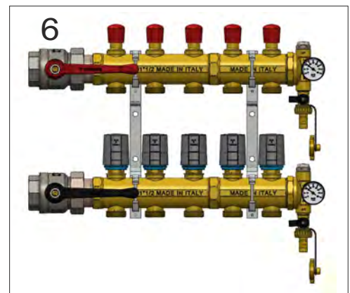
ART. 1436N06 Per tubo PE-X For PE-X pipe
