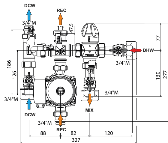
4738KR Anti-scald thermostatic kit with recirculation
