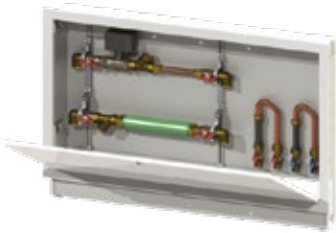
6501C0132V2 Pre-installation metal housing for "FLOOR DN32" system, with 2-way zone valve. Setup stubs included.
