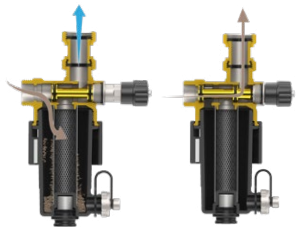
By-pass open: filter on
