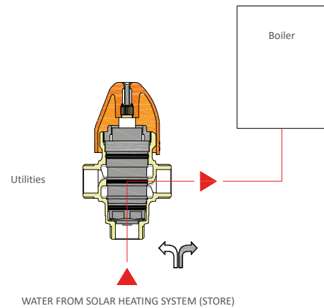
Diagram 2: T > diverter calibration value
